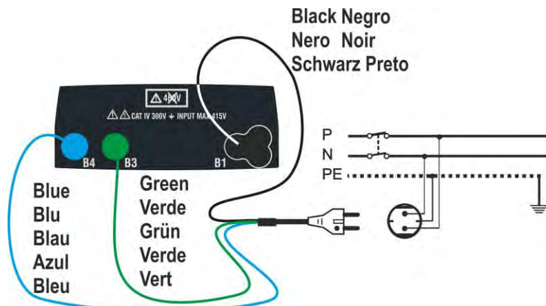
Fig. 8: Instrument connection through mains plug
