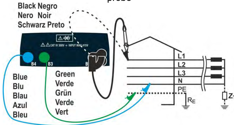
Fig. 30: L1-PE measurement for IT systems by means of single cables and remote probe
