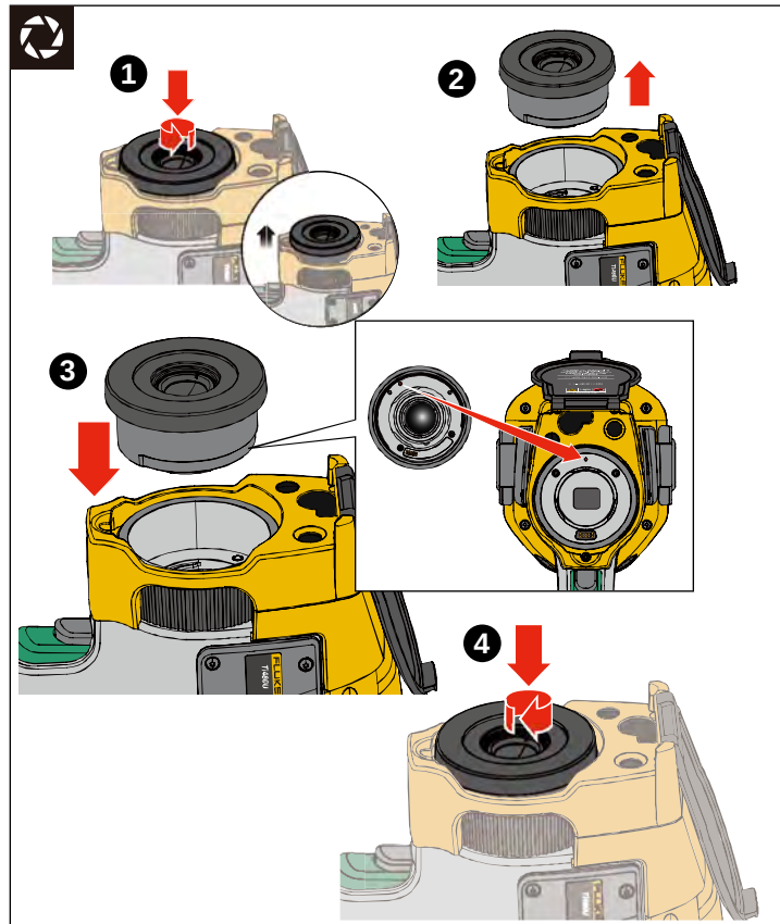
Figure 18. Replace a Lens
