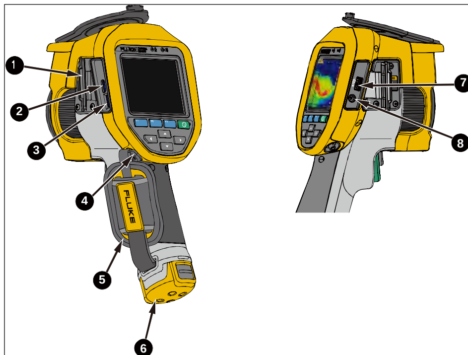
Figure 4. Connections and Power Supply
